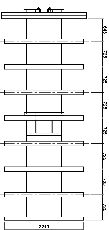
PLAN VIEW ON 'X' MEMBERS
