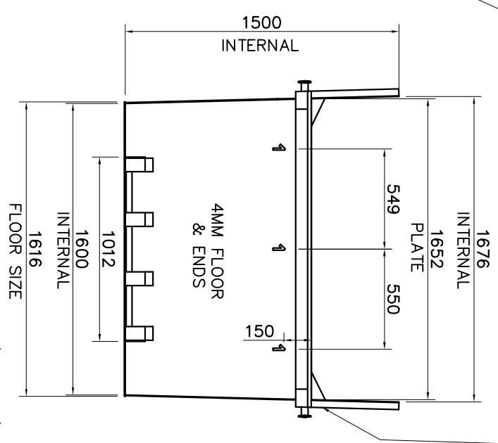
FIT WRAP AROUND PLATES AND CORNER GUSSETS
