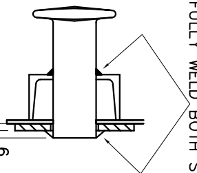
LIFTING LUG FITTING DETAIL SCALE 1 : 3
